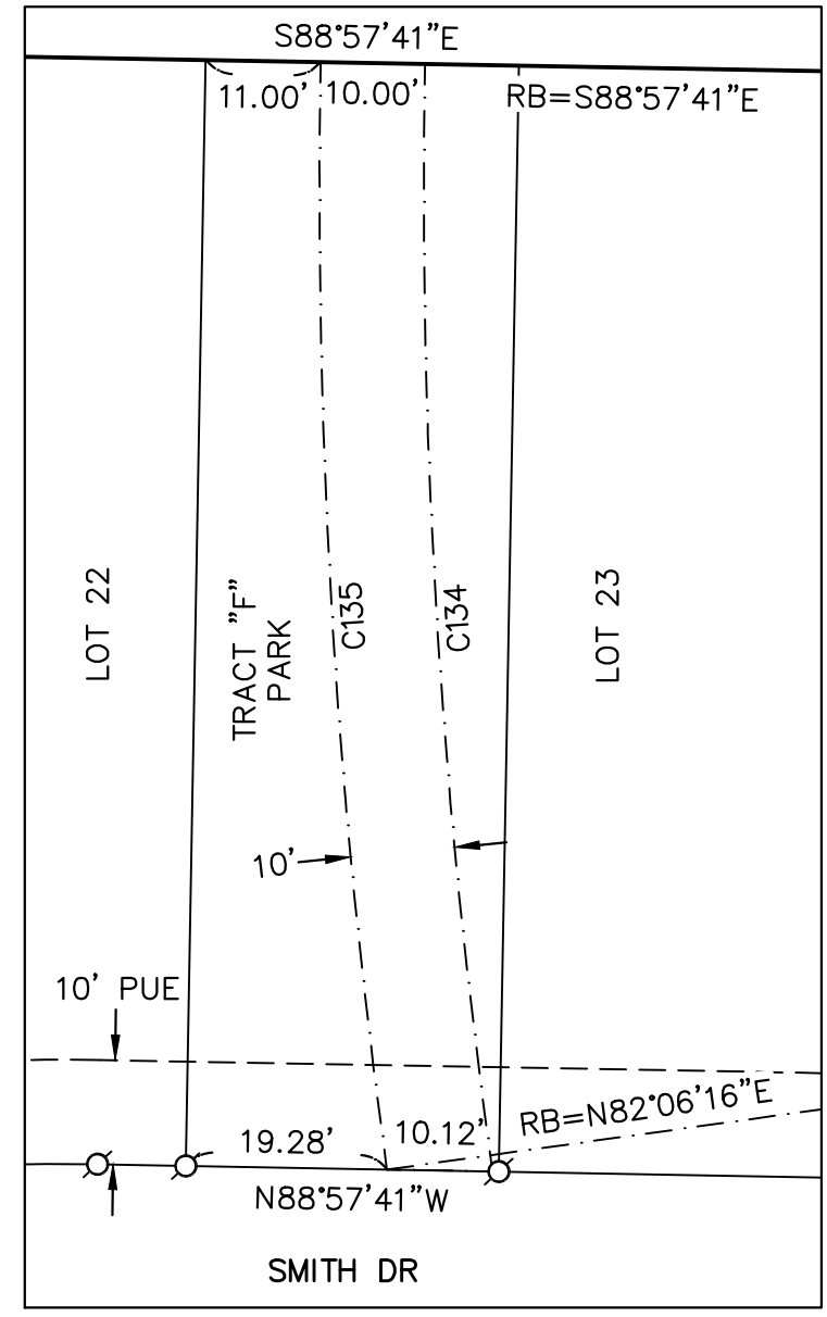
DETAIL "M" SCALE: 1" = 20' (10' DRAINAGE EASEMENT PER V. 616, P. 32, M.C.D.R.)
