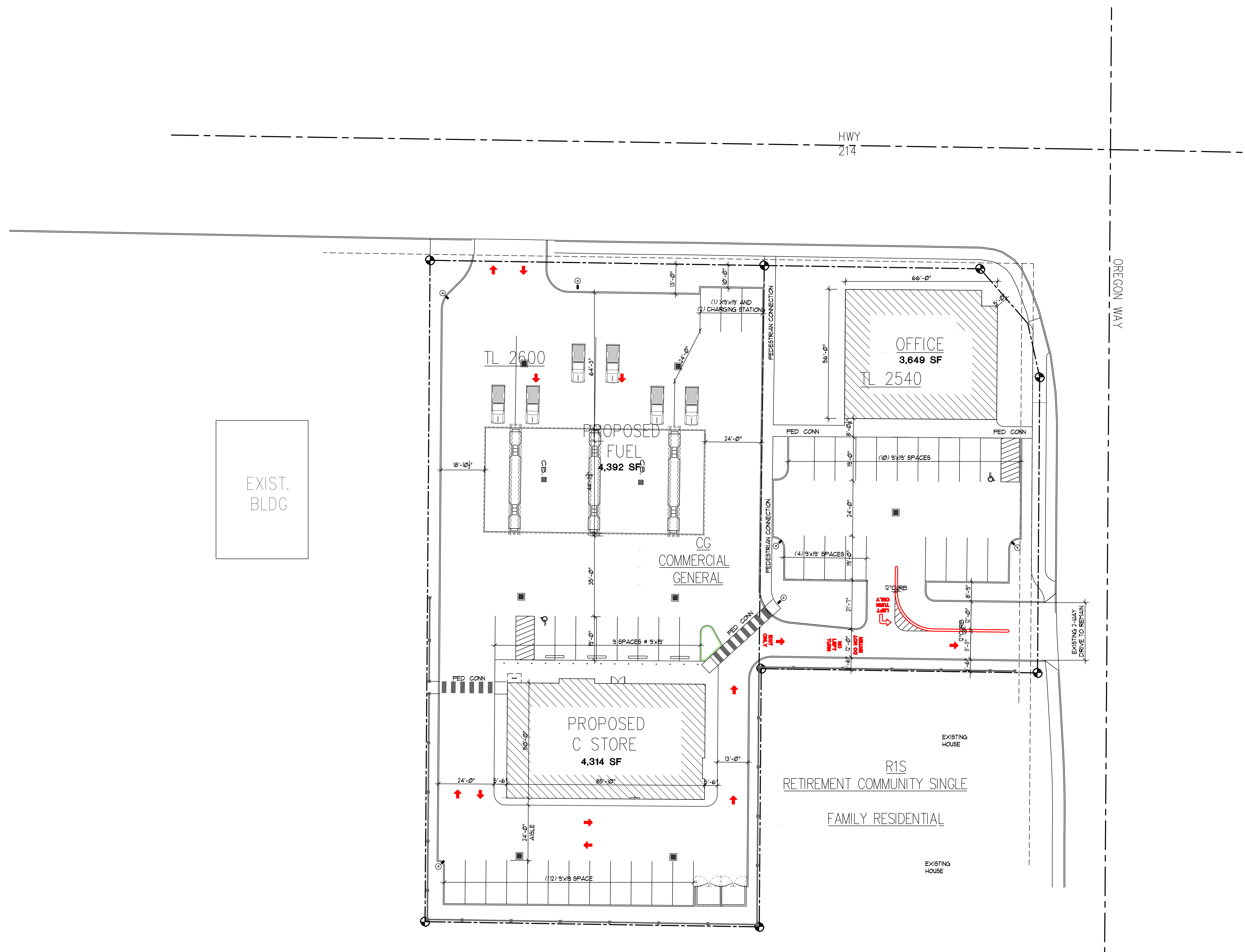
REVISED SITE PLAN SCALE: 1" = 20'
