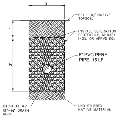
SOAKAGE TRENCH DETAIL 1 SCALE: NTS C-2
