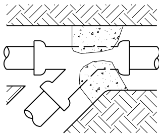
WYE
