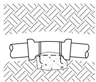
VERTICAL BEND
