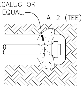
STRADDLE BLOCK
