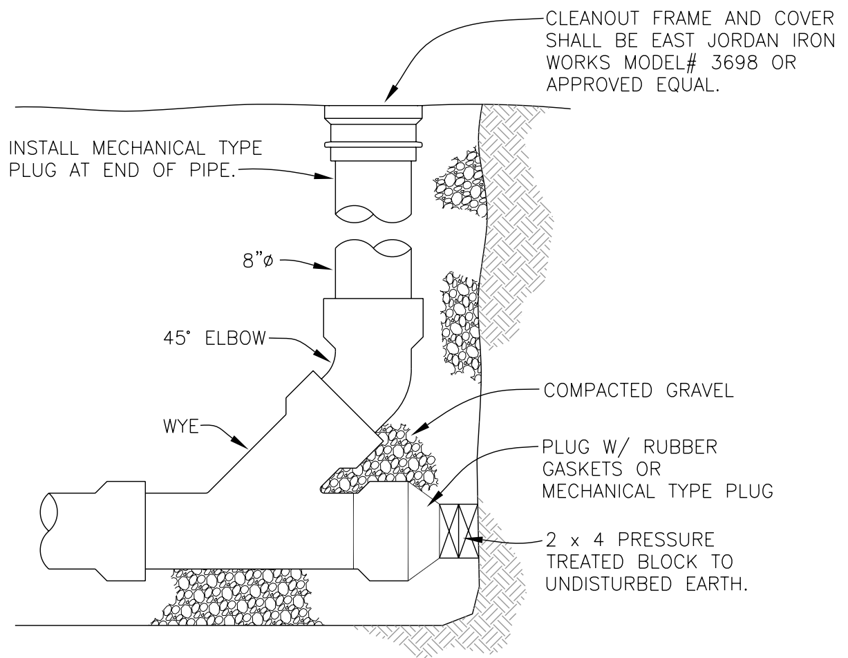
ELEVATION VIEW
